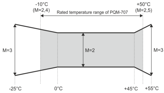
Fig. 77. Basic uncertainty multiplier M as a function of ambient temperature (does not apply to the reference conditions).
